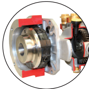
Vibroflex Coupling Cutaway
