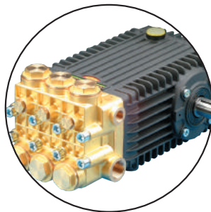
Interpump 66 Series
